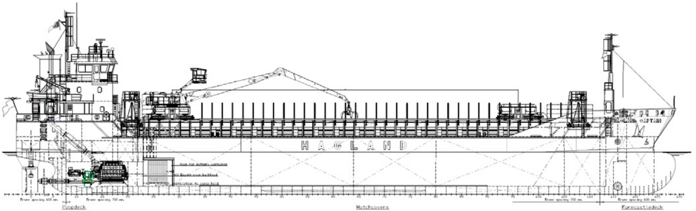
LOADING SALT
